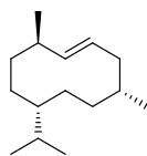
Germacrene D
